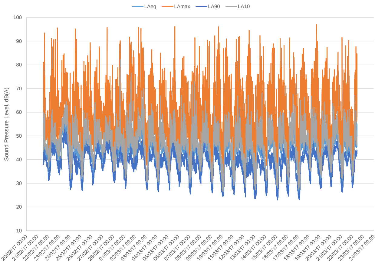
LT4 - Sound Pressure Level - Time Level Trace
